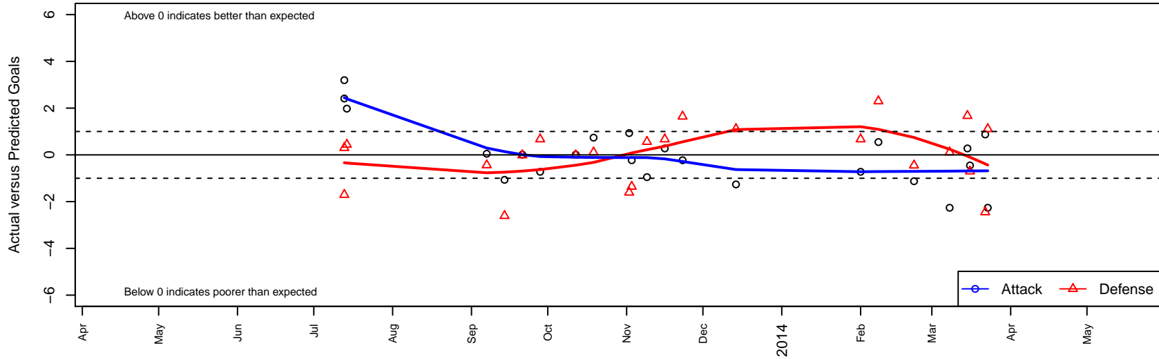
FC Crush Classic B01 Dots are actual minus expected GF (blue circles) and GA (red triangles). Blue line is smoothed change in attack strength. Red is smoothed change in defense strength.
